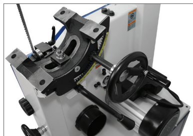
QUICK-LOCK CAST IRON TRUNNION SYSTEM
